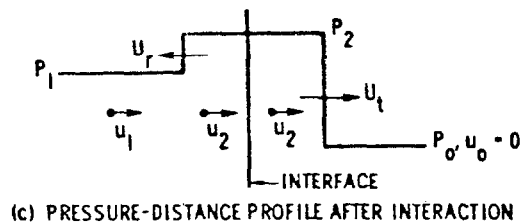
Fig 2 Transmission of a plane shock wave into a material of higher impedance
